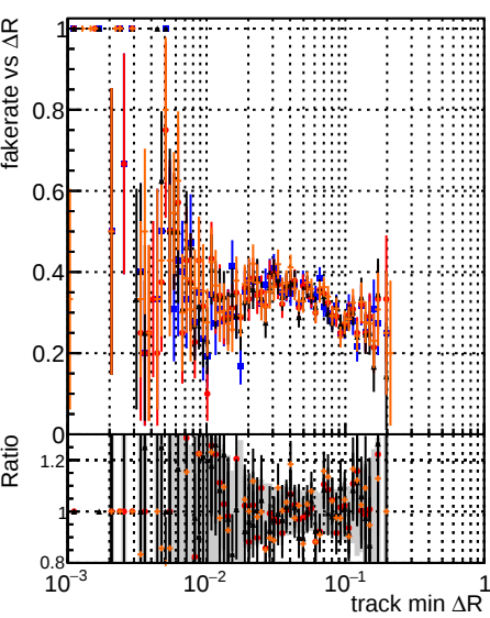
DOM original step2 ttbar phase1-newgeom DOM pixel CDF template step2 ttbar phase1-newgeom DOM pixel CDF template chi-squares step2 ttbar phase1-newgeom test
