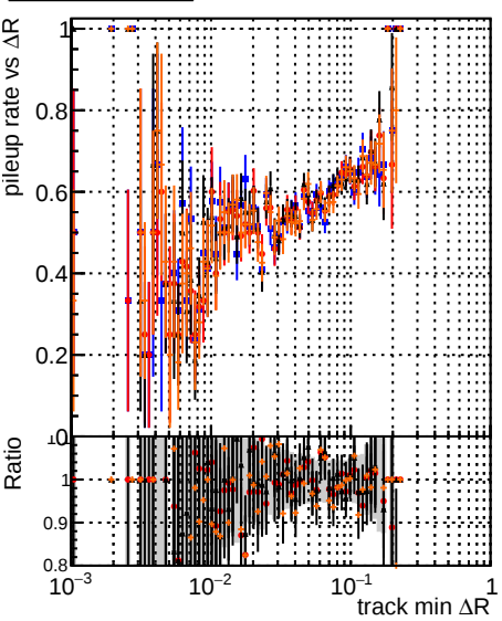
DOM original step2 ttbar phase1-newgeom DOM pixel CDF template step2 ttbar phase1-newgeom DOM pixel CDF template chi-squares step2 ttbar phase1-newgeom test
