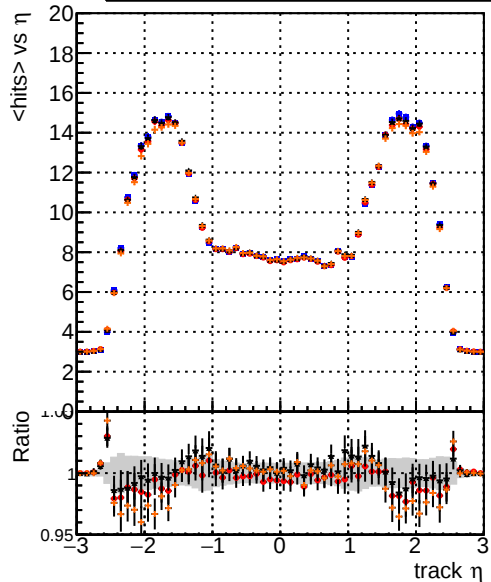
mean hits Legend: Blue line: DQM_original_step2_ttbar-phase1-newgeom Red line: DQM_pixelCPETemplate_step2_ttbar-phase1-newgeom Black line: DQM_pixelCPETemplateCutChiSquare5_step2_ttbar-phase1-newgeom Orange line: DQM_pixelCPETemplateCutChiSquare5_step2_ttbar-phase1-newgeom_test
