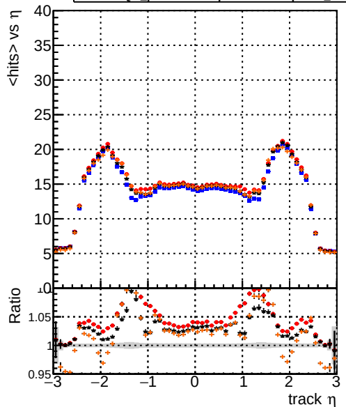
mean hits vs \eta Legend: Blue line: DQM_original_step2_ttbar-phase1-newgeom Red line: DQM_pixelCPETemplate_step2_ttbar-phase1-newgeom Black line: DQM_pixelCPETemplateCutChiSquare5_step2_ttbar-phase1-newgeom Orange line: DQM_pixelCPETemplateCutChiSquare5_step2_ttbar-phase1-newgeom_test
