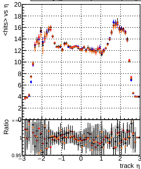
mean hits — DQM_original_step2_ttbar-phase1-newgeom — DQM_pixelCPEtemplate_step2_ttbar-phase1-newgeom — DQM_pixelCPEtemplateCutChiSquare5_step2_ttbar-phase1-newgeom — DQM_pixelCPEtemplateCutChiSquare5_step2_ttbar-phase1-newgeom_test
