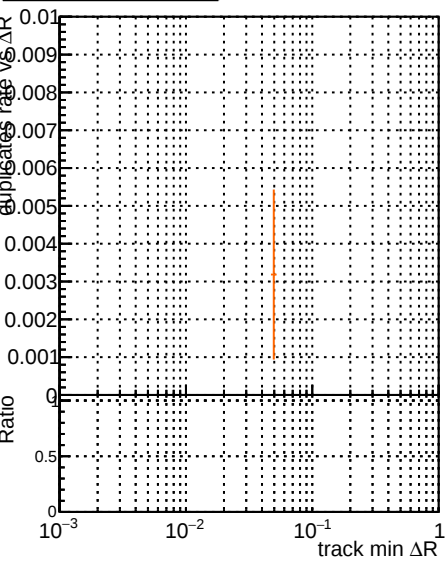
DOM original step2 ttbar phase1-newgeom DOM pixel CDF template step2 ttbar phase1-newgeom DOM pixel CDF template cut chi squares step2 ttbar phase1-newgeom test
