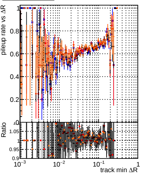
DOM original step2 ttbar phase1-newgeom DOM pixel CDF template step2 ttbar phase1-newgeom DOM pixel CDF template cut chi squares step2 ttbar phase1-newgeom test
