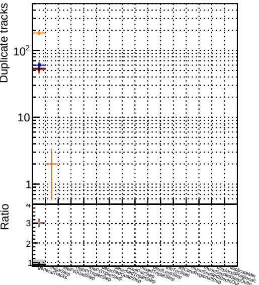
Number Legend Model 1 DQM pixelCPETemplateCutChiSquare5_step2_ttbar-phase1-newgeom 2 DQM pixelCPETemplateCutChiSquare5_step2_ttbar-phase1-newgeom_test
