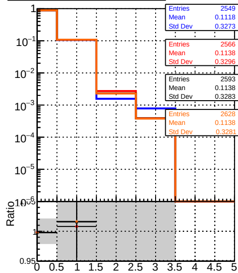
— DQM_original_step2_ttbar-phase1-newgeom — DQM_pixelCPETemplate_step2_ttbar-phase1-newgeom — DQM_pixelCPETemplateCutChiSquare5_step2_ttbar-phase1-newgeom — DQM_pixelCPETemplateCutChiSquare5_step2_ttbar-phase1-newgeom_test
