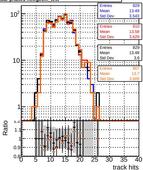
— DQM_original_step2_ttbar-phase1-newgeom — DQM_pixelCPETemplate_step2_ttbar-phase1-newgeom — DQM_pixelCPETemplateCutChiSquare5_step2_ttbar-phase1-newgeom — DQM_pixelCPETemplateCutChiSquare5_step2_ttbar-phase1-newgeom_test
