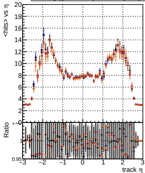
mean hits vs \eta — DQM_original_step2_ttbar-phase1-newgeom — DQM_pixelCPETemplate_step2_ttbar-phase1-newgeom — DQM_pixelCPETemplateCutChiSquare5_step2_ttbar-phase1-newgeom — DQM_pixelCPETemplateCutChiSquare5_step2_ttbar-phase1-newgeom_test
