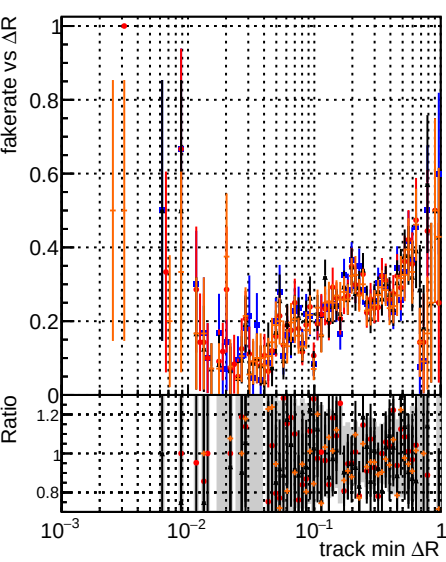
Fake rate vs \Delta R (track, jet) | Duplicates Rate vs \Delta R (track, jet) | Pileup rate vs \Delta R (track, jet) Legend: DOM original (blue squares), DOM pixel (red circles), DOM template (black triangles), DOM cut (orange squares), DOM original step2 (blue squares), DOM pixel step2 (red circles), DOM template step2 (black triangles), DOM cut step2 (orange squares), DOM original tbar phase1 (blue squares), DOM pixel tbar phase1 (red circles), DOM template tbar phase1 (black triangles), DOM cut tbar phase1 (orange squares), DOM original newgeom (blue squares), DOM pixel newgeom (red circles), DOM template newgeom (black triangles), DOM cut newgeom (orange squares).
