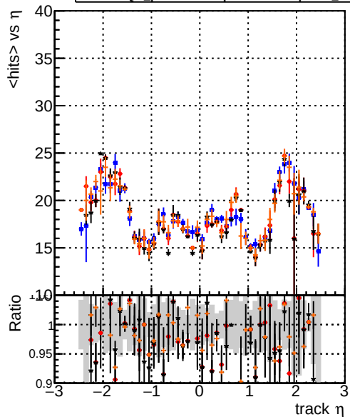
mean hits vs \eta Legend: - DQM_original_step2_ttbar-phase1-newgeom (blue line) - DQM_pixelCPETemplate_step2_ttbar-phase1-newgeom (red line) - DQM_pixelCPETemplateCutChiSquare5_step2_ttbar-phase1-newgeom (black line) - DQM_pixelCPETemplateCutChiSquare5_step2_ttbar-phase1-newgeom_test (orange line)
