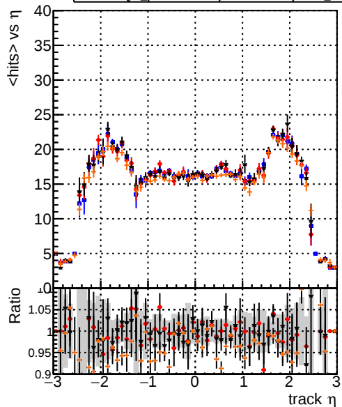
mean hits DQM_original_step2_ttbar-phase1-newgeom DQM_pixelCPETemplate_step2_ttbar-phase1-newgeom DQM_pixelCPETemplateCutChiSquare5_step2_ttbar-phase1-newgeom DQM_pixelCPETemplateCutChiSquare5_step2_ttbar-phase1-newgeom_test
