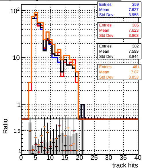
mean hit — DQM_original_step2_ttbar-phase1-newgeom — DQM_pixelCPETemplate_step2_ttbar-phase1-newgeom — DQM_pixelCPETemplateCutChiSquare5_step2_ttbar-phase1-newgeom — DQM_pixelCPETemplateCutChiSquare5_step2_ttbar-phase1-newgeom_test
