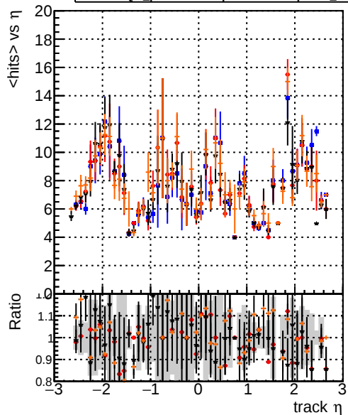
mean hit — DQM_original_step2_ttbar-phase1-newgeom — DQM_pixelCPETemplate_step2_ttbar-phase1-newgeom — DQM_pixelCPETemplateCutChiSquare5_step2_ttbar-phase1-newgeom — DQM_pixelCPETemplateCutChiSquare5_step2_ttbar-phase1-newgeom_test
