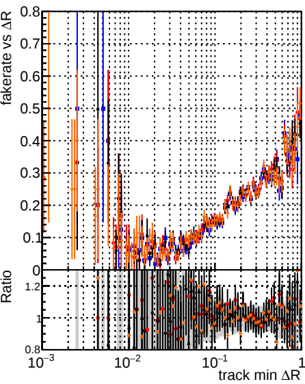
Fake rate vs \Delta R(\text{track, jet}) DQM original_step2_ttbar_phase1-newgeom DQM pixel_CDF_template_step2_ttbar_phase1-newgeom DQM pixel_CDF_template_cut_chi_squares_step2_ttbar_phase1-newgeom test
