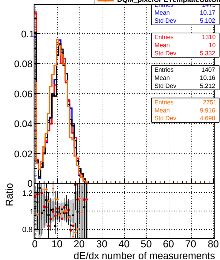
— DQM_original_step2_ttbare-phase1-newgeom — DQM_pixelCPETemplate_step2_ttbare-phase1-newgeom — DQM_pixelCPETemplateCutChiSquare5_step2_ttbare-phase1-newgeom — DQM_pixelCPETemplateCutChiSquare5_step2_ttbare-phase1-newgeom_test
