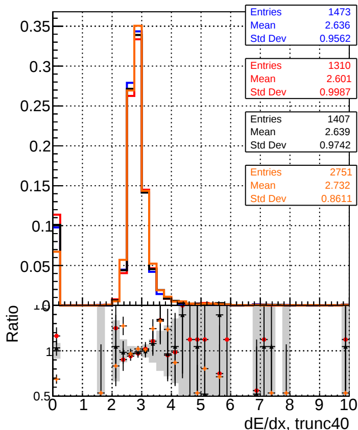
— DQM_original_step2_ttbare-phase1-newgeom — DQM_pixelCPETemplate_step2_ttbare-phase1-newgeom — DQM_pixelCPETemplateCutChiSquare5_step2_ttbare-phase1-newgeom — DQM_pixelCPETemplateCutChiSquare5_step2_ttbare-phase1-newgeom_test
