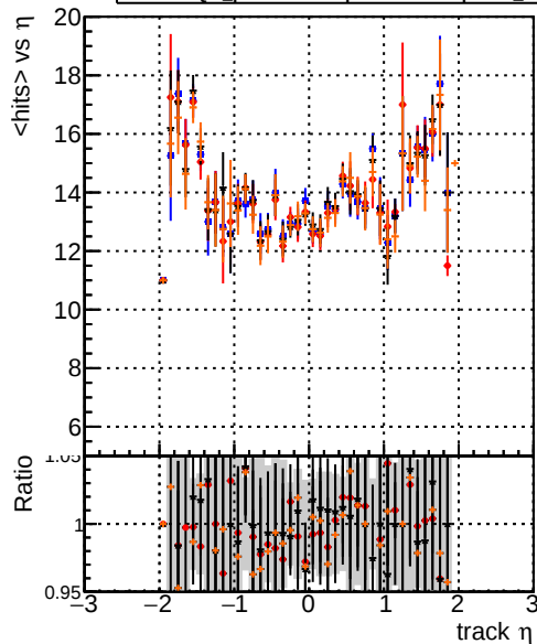
DQM_original_step2_ttbar-phase1-newgeom DQM_pixelCPETemplate_step2_ttbar-phase1-newgeom DQM_pixelCPETemplateCutChiSquare5_step2_ttbar-phase1-newgeom DQM_pixelCPETemplateCutChiSquare5_step2_ttbar-phase1-newgeom_test
