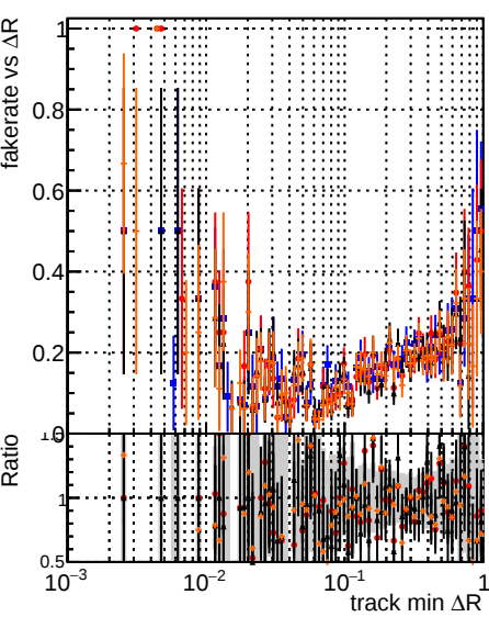
Fake rate vs \Delta R(\text{track, jet}) DOM original_step2_ttbar-phase1-newgeom DOM pixelCUT+template_step2_ttbar-phase1-newgeom DOM pixelCUT+template+chiSquares_step2_ttbar-phase1-newgeom DOM pixelCUT+template+chiSquares_step2_ttbar-phase1-newgeom test
