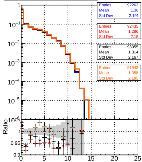
mean hit — DQM_original_step2_ttbar-phase1-newgeom — DQM_pixelCPETemplate_step2_ttbar-phase1-newgeom — DQM_pixelCPETemplateCutChiSquare5_step2_ttbar-phase1-newgeom — DQM_pixelCPETemplateCutChiSquare5_step2_ttbar-phase1-newgeom_test
