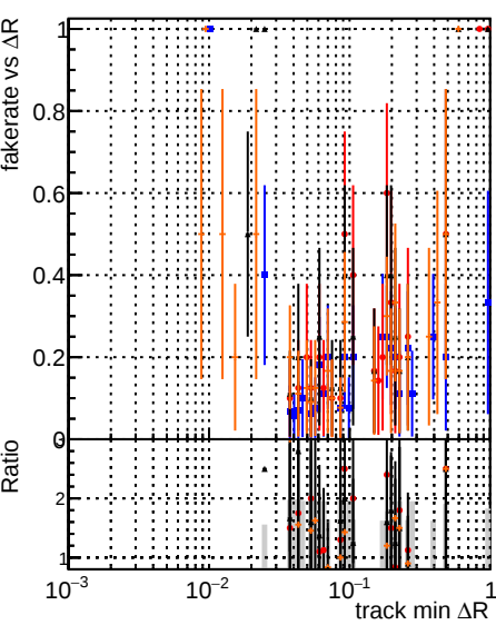
Fake rate vs \Delta R(\text{track, jet}) DOM original_step2_ttbar-phase1-newgeom DOM pixel_CDF-template_step2_ttbar-phase1-newgeom DOM pixel_CDF-template_chi-squares_step2_ttbar-phase1-newgeom test
