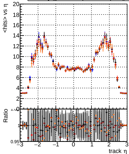
mean hit DQM_original_step2_ttbar-phase1-newgeom DQM_pixelCPETemplate_step2_ttbar-phase1-newgeom DQM_pixelCPETemplateCutChiSquare5_step2_ttbar-phase1-newgeom DQM_pixelCPETemplateCutChiSquare5_step2_ttbar-phase1-newgeom_test
