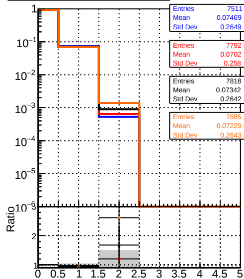
mean hit DQM_original_step2_ttbar-phase1-newgeom DQM_pixelCPETemplate_step2_ttbar-phase1-newgeom DQM_pixelCPETemplateCutChiSquare5_step2_ttbar-phase1-newgeom DQM_pixelCPETemplateCutChiSquare5_step2_ttbar-phase1-newgeom_test
