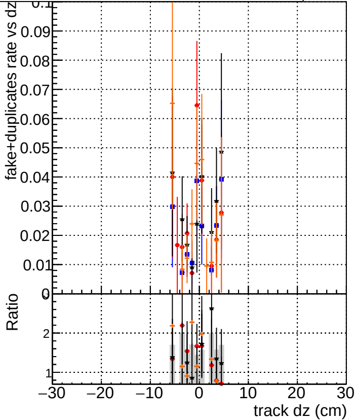
DQM_original_step2_ttbar-phase1-newgeom DQM_pixelCPETemplate_step2_ttbar-phase1-newgeom DQM_pixelCPETemplateCutChiSquare5_step2_ttbar-phase1-newgeom DQM_pixelCPETemplateCutChiSquare5_step2_ttbar-phase1-newgeom_test
