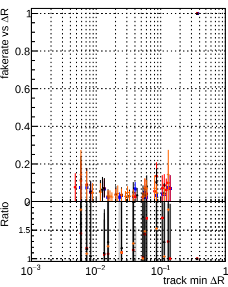
Legend: DOM original_step2_ttbare1-newgeom DOM pixelCDE template_step2_ttbare1-newgeom DOM pixelCDE template_chi2_squares_step2_ttbare1-newgeom test DOM pixelCDE template_chi2_squares_step2_ttbare1-newgeom
