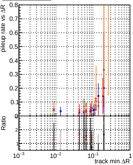
Legend: DOM original_step2_ttbare1-newgeom DOM pixelCDE template_step2_ttbare1-newgeom DOM pixelCDE template_chi2_squares_step2_ttbare1-newgeom test DOM pixelCDE template_chi2_squares_step2_ttbare1-newgeom
