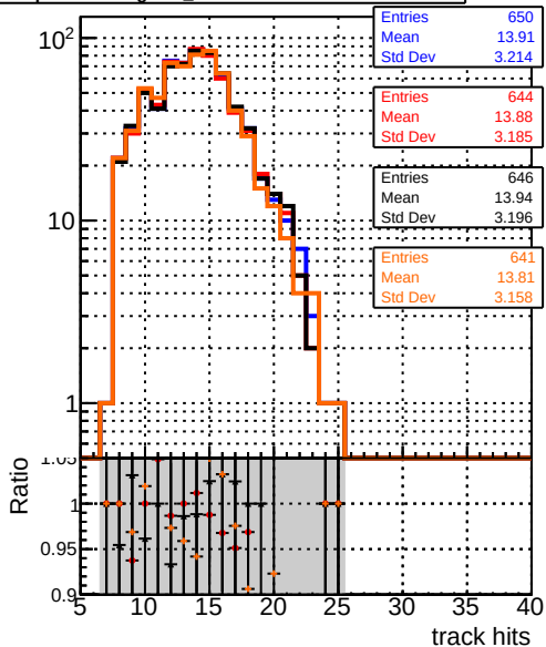
mean hit DQM_original_step2_ttbar-phase1-newgeom DQM_pixelCPETemplate_step2_ttbar-phase1-newgeom DQM_pixelCPETemplateCutChiSquare5_step2_ttbar-phase1-newgeom DQM_pixelCPETemplateCutChiSquare5_step2_ttbar-phase1-newgeom_test
