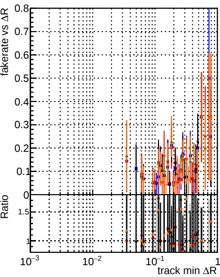
Fake rate vs \Delta R(\text{track, jet}) Legend: DOM original_step2_ttbar_phase1-newgeom, DOM pixelCBTemplate_step2_ttbar_phase1-newgeom, DOM pixelCBTemplate_chiSquares_step2_ttbar_phase1-newgeom, DOM pixelCBTemplate_chiSquares_step2_ttbar_phase1-newgeom test
