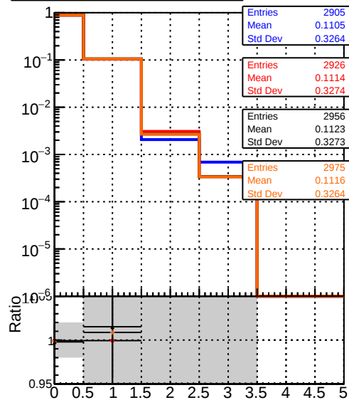
mean hits — DQM_original_step2_ttbar-phase1-newgeom — DQM_pixelCPETemplate_step2_ttbar-phase1-newgeom — DQM_pixelCPETemplateCutChiSquare5_step2_ttbar-phase1-newgeom — DQM_pixelCPETemplateCutChiSquare5_step2_ttbar-phase1-newgeom_test
