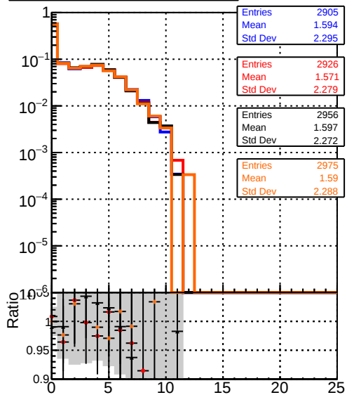
mean hits — DQM_original_step2_ttbar-phase1-newgeom — DQM_pixelCPETemplate_step2_ttbar-phase1-newgeom — DQM_pixelCPETemplateCutChiSquare5_step2_ttbar-phase1-newgeom — DQM_pixelCPETemplateCutChiSquare5_step2_ttbar-phase1-newgeom_test
