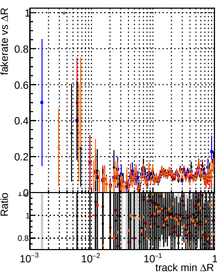
Fake rate vs \Delta R(\text{track, jet}) DOM original_step2_ttbarm-phase1-newgeom DOM pixel_CDF-template_step2_ttbarm-phase1-newgeom DOM pixel_CDF-template_CutSquares_step2_ttbarm-phase1-newgeom test
