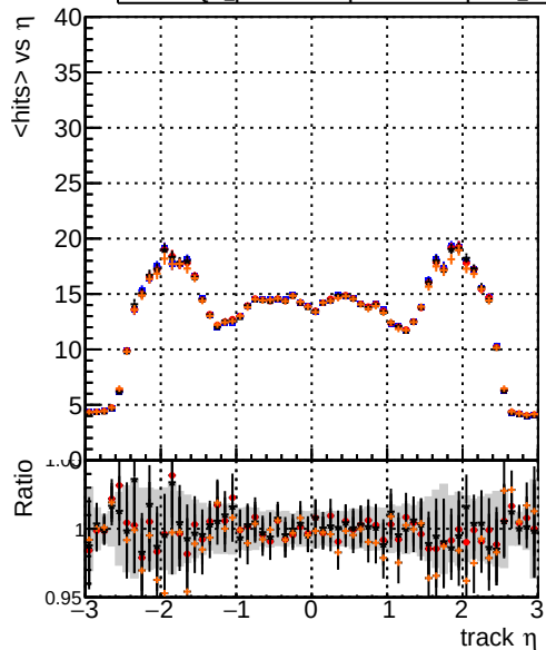
DQM_original_step2_ttbar-phase1-newgeom DQM_pixelCPETemplate_step2_ttbar-phase1-newgeom DQM_pixelCPETemplateCutChiSquare5_step2_ttbar-phase1-newgeom DQM_pixelCPETemplateCutChiSquare5_step2_ttbar-phase1-newgeom_test
