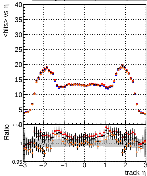
mean hit — DQM_original_step2_ttbar-phase1-newgeom — DQM_pixelCPETemplate_step2_ttbar-phase1-newgeom — DQM_pixelCPETemplateCutChiSquare5_step2_ttbar-phase1-newgeom — DQM_pixelCPETemplateCutChiSquare5_step2_ttbar-phase1-newgeom_test
