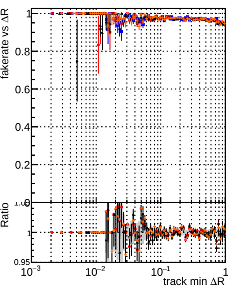
Fake rate vs \Delta R(\text{track, jet}) DOM original step2 ttbar phase1-newgeom DOM pixelCPE template step2 ttbar phase1-newgeom DOM pixelCPE template cut chi-squares step2 ttbar phase1-newgeom test
