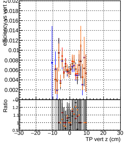
Efficiency vs vert z —•— DQM_original_step2_ttbar-phase1-newgeom —•— DQM_pixelCPETemplate_step2_ttbar-phase1-newgeom —•— DQM_pixelCPETemplateCutChiSquare5_step2_ttbar-phase1-newgeom —•— DQM_pixelCPETemplateCutChiSquare5_step2_ttbar-phase1-newgeom_test
