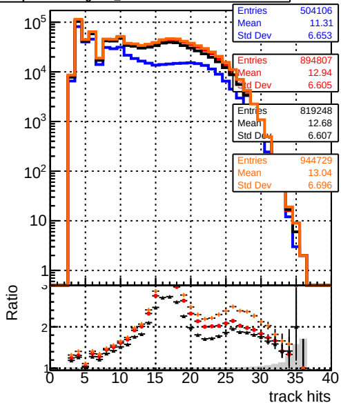
mean hits — DQM_original_step2_ttbar-phase1-newgeom — DQM_pixelCPETemplate_step2_ttbar-phase1-newgeom — DQM_pixelCPETemplateCutChiSquare5_step2_ttbar-phase1-newgeom — DQM_pixelCPETemplateCutChiSquare5_step2_ttbar-phase1-newgeom_test
