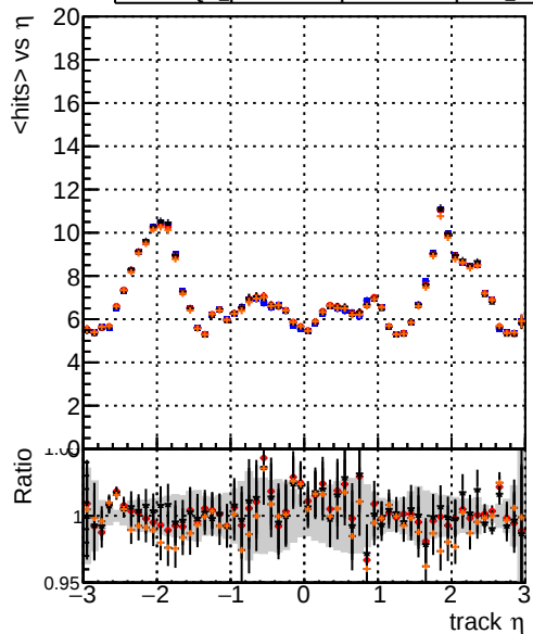
mean hits vs \eta Legend: - DQM_original_step2_ttbar-phase1-newgeom - DQM_pixelCPETemplate_step2_ttbar-phase1-newgeom - DQM_pixelCPETemplateCutChiSquare5_step2_ttbar-phase1-newgeom - DQM_pixelCPETemplateCutChiSquare5_step2_ttbar-phase1-newgeom_test
