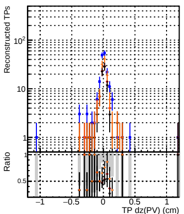
N of associated tracks (simToReco) vs dz(PV) zoomed
