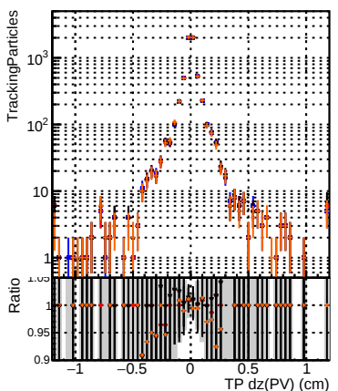
N of simulated tracks vs dz(PV) zoomed
