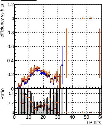
Efficiency vs hit DQM_original_step2_ttbar-phase1-newgeom DQM_pixelCPETemplate_step2_ttbar-phase1-newgeom DQM_pixelCPETemplateCutChiSquare5_step2_ttbar-phase1-newgeom DQM_pixelCPETemplateCutChiSquare5_step2_ttbar-phase1-newgeom_test
