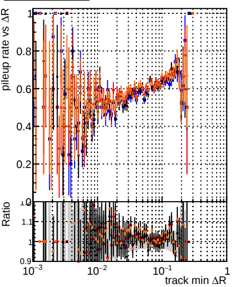
DOM original_step2_ttbar_phase1-newgeom DOM pixelCUT_template_step2_ttbar_phase1-newgeom DOM pixelCUT_chiSquares_step2_ttbar_phase1-newgeom DOM templateCUT_chiSquares_step2_ttbar_phase1-newgeom test
