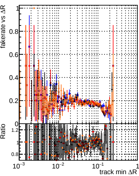
DOM original_step2_ttbar_phase1-newgeom DOM pixelCUT_template_step2_ttbar_phase1-newgeom DOM pixelCUT_chiSquares_step2_ttbar_phase1-newgeom DOM templateCUT_chiSquares_step2_ttbar_phase1-newgeom test
