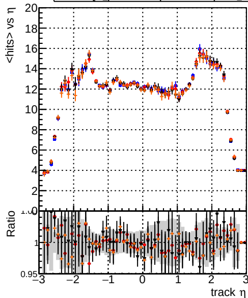
mean hits vs \eta — DQM_original_step2_ttbar-phase1-newgeom — DQM_pixelCPEtemplate_step2_ttbar-phase1-newgeom — DQM_pixelCPEtemplateCutChiSquare5_step2_ttbar-phase1-newgeom — DQM_pixelCPEtemplateCutChiSquare5_step2_ttbar-phase1-newgeom_test
