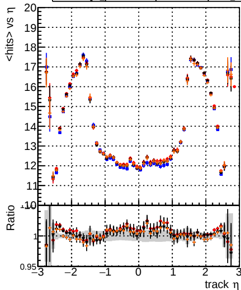
mean hits vs \eta DQM_original_step2_ttbar-phase1-newgeom DQM_pixelCPETemplate_step2_ttbar-phase1-newgeom DQM_pixelCPETemplateCutChiSquare5_step2_ttbar-phase1-newgeom DQM_pixelCPETemplateCutChiSquare5_step2_ttbar-phase1-newgeom_test
