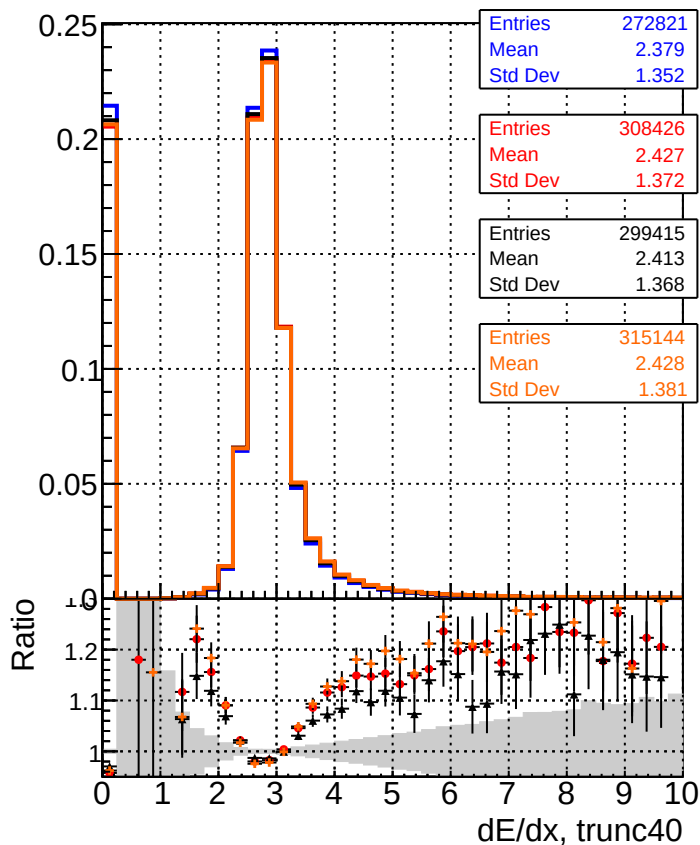
— DQM_original_step2_ttbbar-phase1-newgeom — DQM_pixelCPETemplate_step2_ttbbar-phase1-newgeom — DQM_pixelCPETemplateCutChiSquare5_step2_ttbbar-phase1-newgeom — DQM_pixelCPETemplateCutChiSquare5_step2_ttbbar-phase1-newgeom_test
