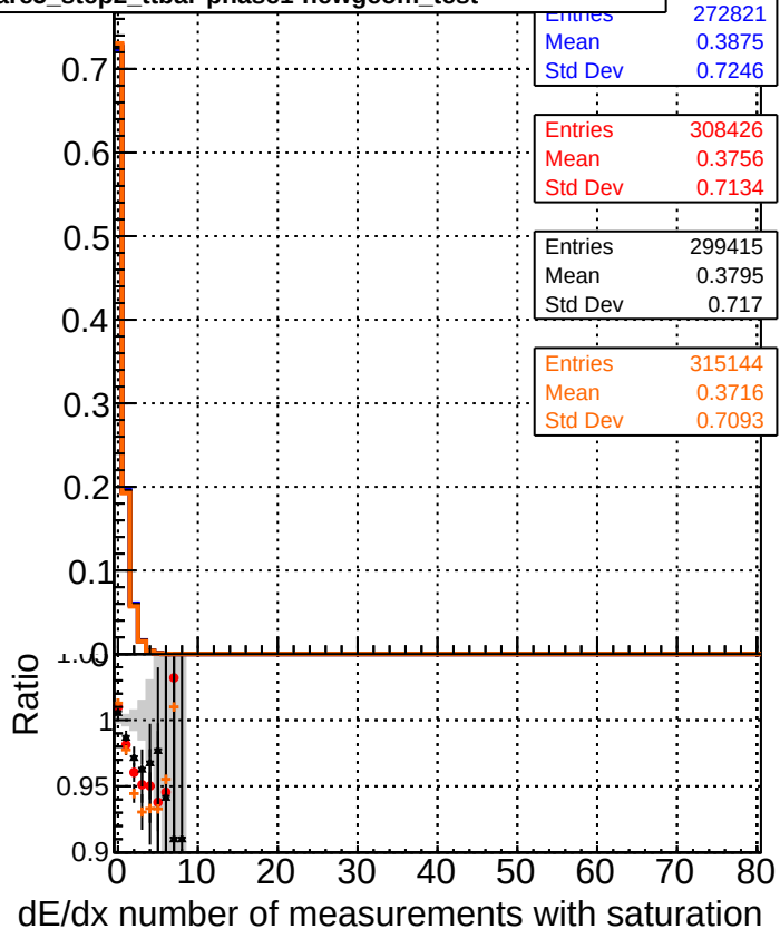
— DQM_original_step2_ttbbar-phase1-newgeom — DQM_pixelCPETemplate_step2_ttbbar-phase1-newgeom — DQM_pixelCPETemplateCutChiSquare5_step2_ttbbar-phase1-newgeom — DQM_pixelCPETemplateCutChiSquare5_step2_ttbbar-phase1-newgeom_test
