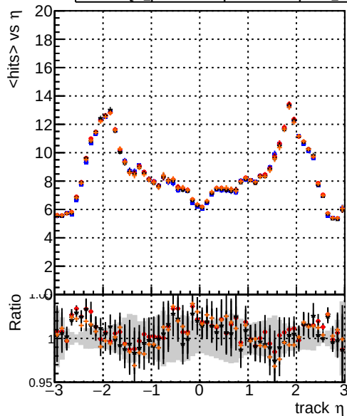
mean hits Legend: Blue line: DQM_original_step2_ttbar-phase1-newgeom Red line: DQM_pixelCPETemplate_step2_ttbar-phase1-newgeom Black line: DQM_pixelCPETemplateCutChiSquare5_step2_ttbar-phase1-newgeom Orange line: DQM_pixelCPETemplateCutChiSquare5_step2_ttbar-phase1-newgeom_test
