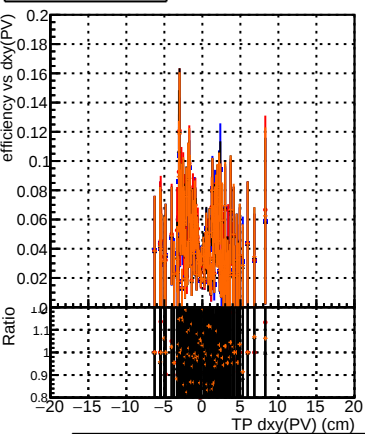
Efficiency vs Dxy(PV) Legend: DQM_original_step2_ttbar-phase1-newgeom DQM_pixelCPETemplate_step2_ttbar-phase1-newgeom DQM_pixelCPETemplateCutChiSquare5_step2_ttbar-phase1-newgeom DQM_pixelCPETemplateCutChiSquare5Test_step2_ttbar-phase1-newgeom
