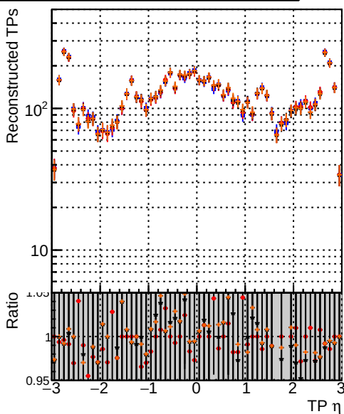
—●— DQM_original_step2_ttbar-phase1-newgeom —●— DQM_pixelCPETemplate_step2_ttbar-phase1-newgeom —●— DQM_pixelCPETemplateCutChiSquare5_step2_ttbar-phase1-newgeom —●— DQM_pixelCPETemplateCutChiSquare5Test_step2_ttbar-phase1-newgeom
