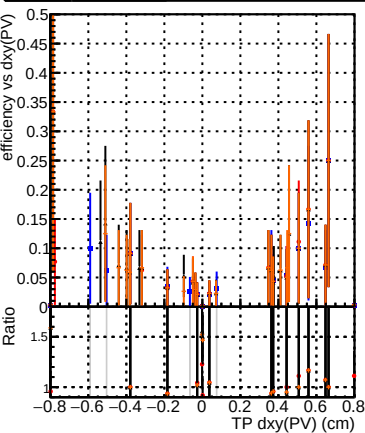
Efficiency vs Dxy(PV) Legend: DQM_original_step2_ttbbar-phase1-newgeom DQM_pixelCPETemplate_step2_ttbbar-phase1-newgeom DQM_pixelCPETemplateCutChiSquare5_step2_ttbbar-phase1-newgeom DQM_pixelCPETemplateCutChiSquare5Test_step2_ttbbar-phase1-newgeom
