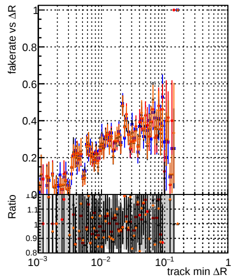
DOM original step2 ttbar-phase1-newgeom DOM pixel CDF template step2 ttbar-phase1-newgeom DOM pixel CDF template cut chi-squares test step2 ttbar-phase1-newgeom
