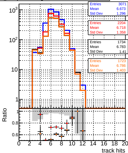
mean hits — DQM_original_step2_ttbar-phase1-newgeom — DQM_pixelCPETemplate_step2_ttbar-phase1-newgeom — DQM_pixelCPETemplateCutChiSquare5_test2_ttbar-phase1-newgeom — DQM_pixelCPETemplateCutChiSquare5Test_step2_ttbar-phase1-newgeom
