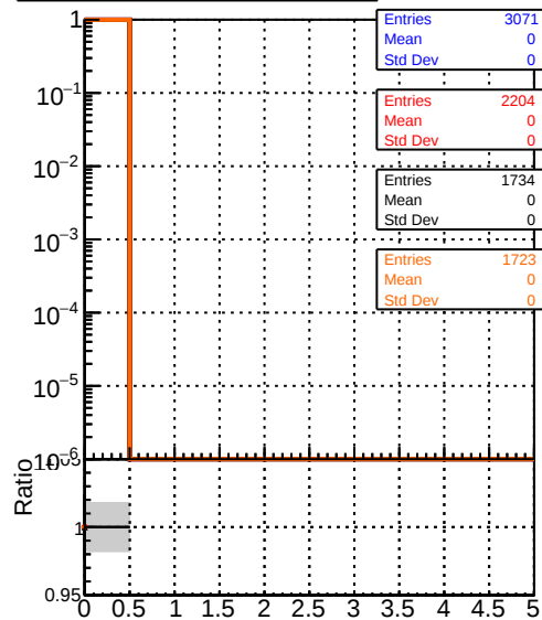
mean hits — DQM_original_step2_ttbar-phase1-newgeom — DQM_pixelCPETemplate_step2_ttbar-phase1-newgeom — DQM_pixelCPETemplateCutChiSquare5_test2_ttbar-phase1-newgeom — DQM_pixelCPETemplateCutChiSquare5Test_step2_ttbar-phase1-newgeom
