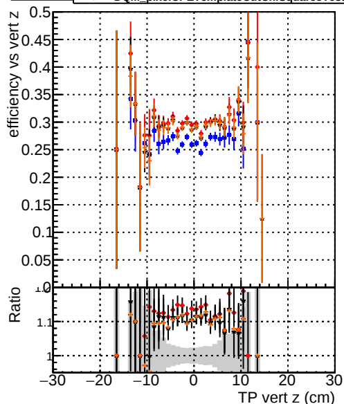
Efficiency vs vert z — DQM_original_step2_ttbar-phase1-newgeom — DQM_pixelCPETemplate_step2_ttbar-phase1-newgeom — DQM_pixelCPETemplateCutChiSquare5_step2_ttbar-phase1-newgeom — DQM_pixelCPETemplateCutChiSquare5Test_step2_ttbar-phase1-newgeom
