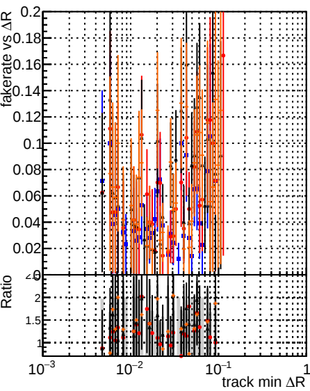
Fake rate vs \Delta R(\text{track, jet}) DQM original_step2_ttbbar-phase1-newgeom DQM pixelCPE-template_step2_ttbbar-phase1-newgeom DQM pixelCPE-template_chi_squares_step2_ttbbar-phase1-newgeom DQM pixelCPE-template_chi_squares_test_step2_ttbbar-phase1-newgeom
