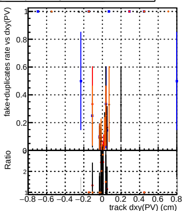
ttbar-phase1-newgeom p2_ttbar-phase1-newgeom
