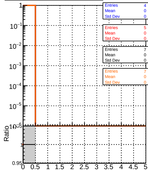
DQM_original_step2_ttbar-phase1-newgeom DQM_pixelCPETemplate_step2_ttbar-phase1-newgeom DQM_pixelCPETemplateCutChiSquare5_step2_ttbar-phase1-newgeom DQM_pixelCPETemplateCutChiSquare5Test_step2_ttbar-phase1-newgeom
