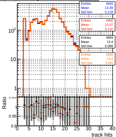
mean hits Legend: Blue line: DQM_original_step2_ttbar-phase1-newgeom Red line: DQM_pixelCPETemplate_step2_ttbar-phase1-newgeom Black line: DQM_pixelCPETemplateCutChiSquare5_test2_ttbar-phase1-newgeom Orange line: DQM_pixelCPETemplateCutChiSquare5Test_step2_ttbar-phase1-newgeom
