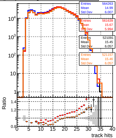
mean hits — DQM_original_step2_ttbar-phase1-newgeom — DQM_pixelCPETemplate_step2_ttbar-phase1-newgeom — DQM_pixelCPETemplateCutChiSquare5_test2_ttbar-phase1-newgeom — DQM_pixelCPETemplateCutChiSquare5Test_step2_ttbar-phase1-newgeom
